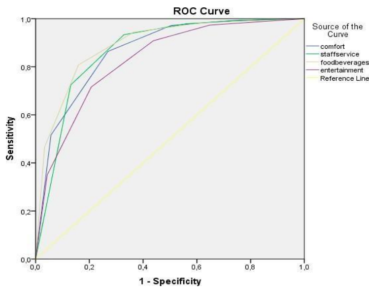
Figure 2. ROC Curve.
